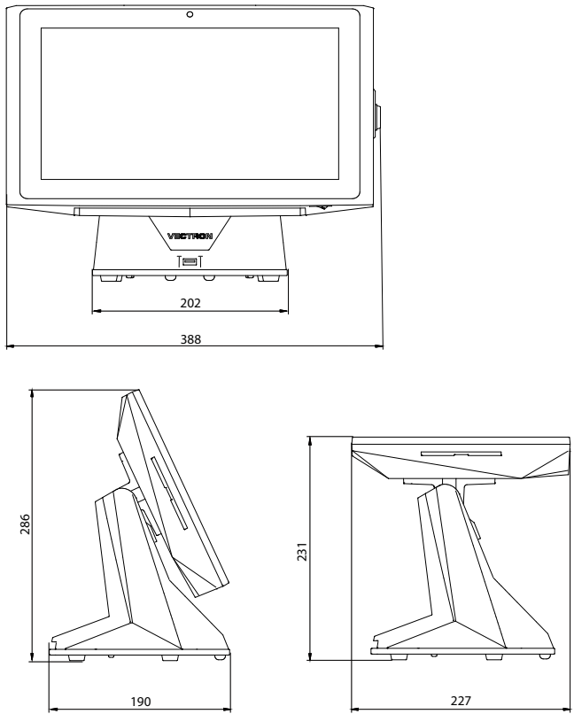
Abb. 4: POS Touch 14 Wide (Maße in Millimetern)
